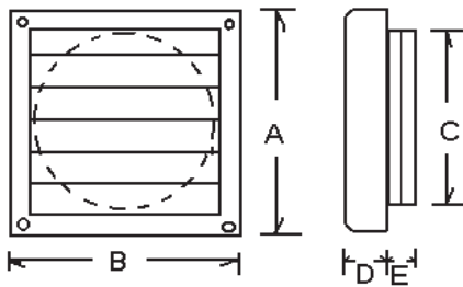
LOUVERED VENTS
